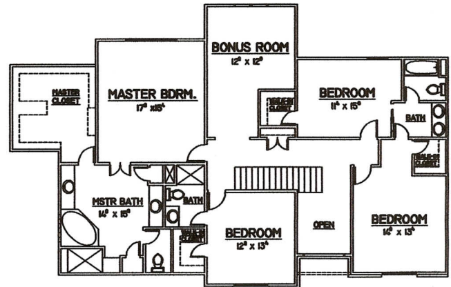
SECOND LEVEL FLOOR PLAN
